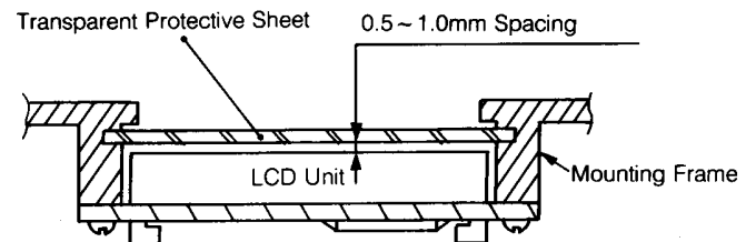
Fig. 10 Sample Design
