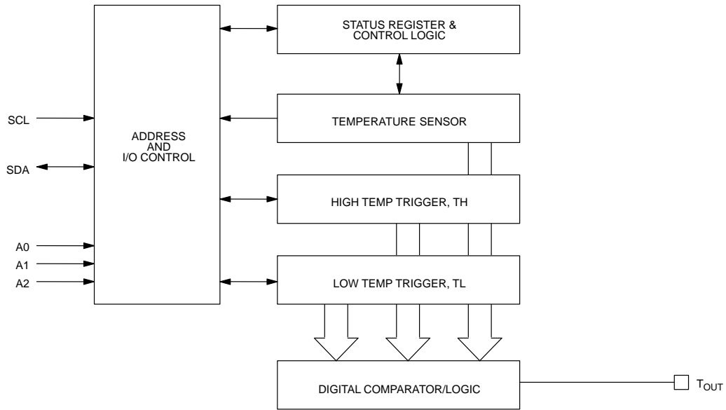
DS1621 FUNCTIONAL BLOCK DIAGRAM Figure 1
