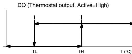
THERMOSTAT OUTPUT OPERATION Figure 3
